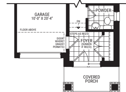
Partial Main Floor ELEVATION C2
