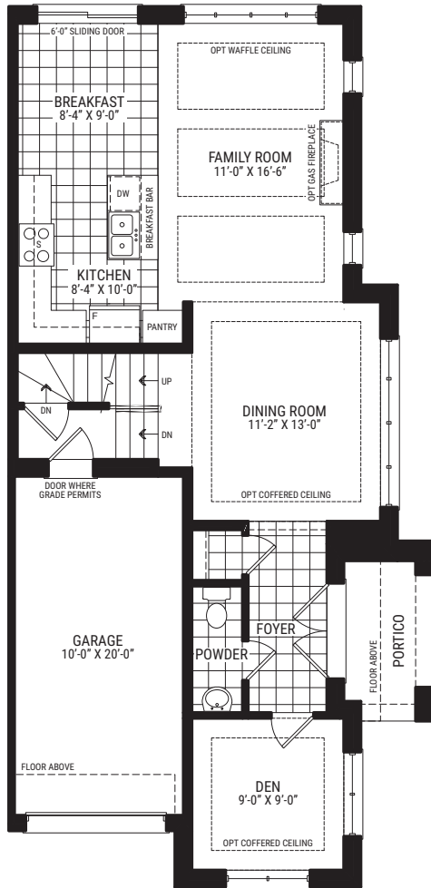
Main Floor ELEVATION A
