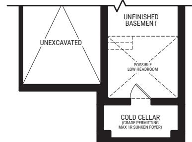
Partial Basement ELEVATION C1 | C2
