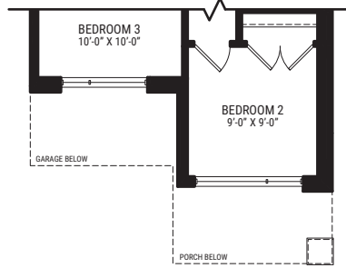
Partial Second Floor ELEVATION C1
