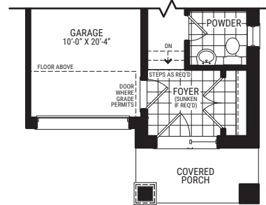
Partial Main Floor ELEVATION C1
