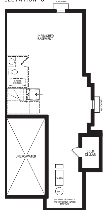
Basement ELEVATION C
